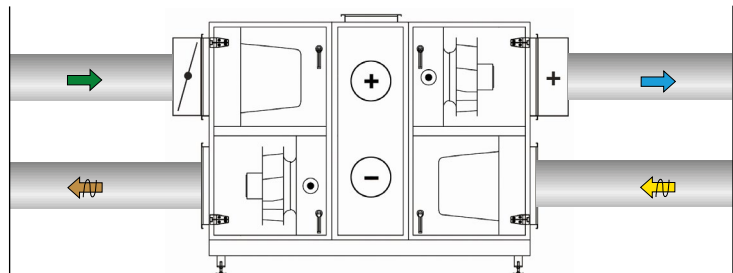
Existing installation
