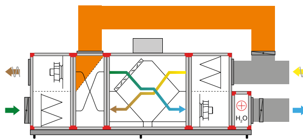
Connection in roof for smoke-bypass with cross-flow section
