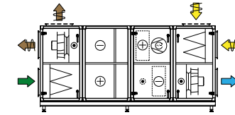
Comb. 12 Run-around coil unit and cooling unit
