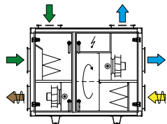
Supply air top
