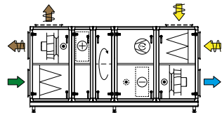
Comb. 3 Cooling unit with cooling recovery
