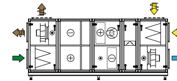
Comb. 14 Run-around coil unit, cooling unit, recirculating unit
