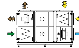
Comb. 11 Run-around coil unit
