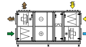
Comb. 13 Run-around coil unit and recirculating unit
