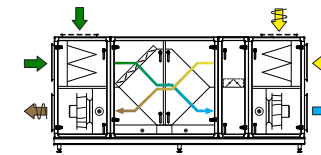
Comb. 9 Counter-flow heat exchanger and recirculating unit
