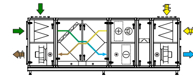
Comb. 10 Counter-flow heat exchanger, cooling unit, recirculating unit
